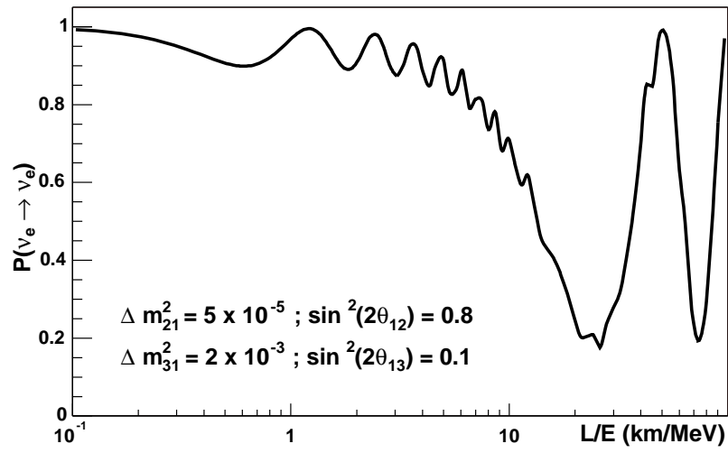
Figure 3: Probability of \nu_e disappearance versus L/E for \theta_{13} at its current upper limit
